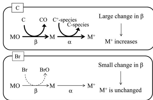
Fig. 5 Schematic diagram of signal enhancement by co-existing carbon. Positively charged carbon species (C + -species) react with the analyte atom (M), and the degree of ionization ( \alpha ) of the analyte increases. Carbon is oxidized by the analyte oxide (MO), and the analyte oxide is reduced to the analyte atom. This process increases the atomization ratio ( \beta ) of the analyte oxide. In contrast, bromine is not oxidized by the analyte oxide.
