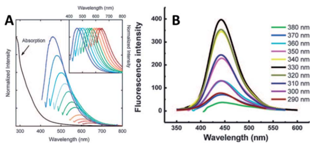
Fig. 12 (A) Absorbance and PL spectra with increasingly longer excitation wavelengths (in 20 nm increments starting from 400 nm) of 5 nm PPEI-EI CQDs in an aqueous solution formed using laser ablation methods (inset shows the normalized PL spectra). Adapted with permission. 2 Copyright 2006, American Chemical Society. (B) PL of 1.9 nm CQDs at different excitation wavelengths of 290–380 nm. Adapted with permission. 19 Copyright 2008, Royal Society of Chemistry.
