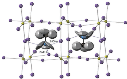
Fig. 1 The unit cell of MAPbI 3 at 100 K viewed close to a -axis showing ADPs as 90% probability ellipsoids; lead yellow, iodine purple, carbon black, nitrogen blue and hydrogen grey.
