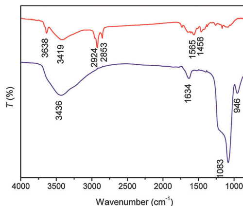
Fig. 25 FTIR spectra of unmodified \text{NaYF}_4:\text{Er} UCNPs (upper red curve) and silica-coated \text{NaYF}_4:\text{Er} UCNPs (lower blue curve). The strong new band at 1083\text{ cm}^{-1} is assigned to stretching vibration of Si-O. Reprinted with permission from ref. 163. Copyright © 2009, American Chemical Society.
