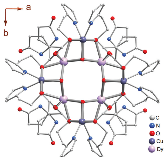
Fig. 1 Molecular structure of complex 1L (along crystallographic c -axis), as obtained from SC-XRD analyses presenting a highly symmetric \text{Dy}(\text{III}) -vertex sharing tetracubane-assemblage based dodecahedral \text{Dy}_4\text{Cu}_8 heterometallic cluster core.
