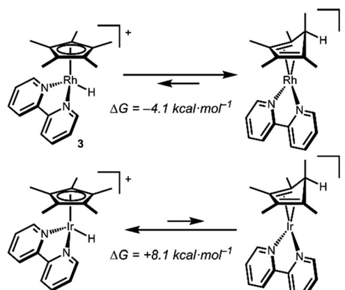
Scheme 3 Free energies for reductive elimination from \text{Cp}^*\text{M}-\text{H} ( \text{M} = \text{Rh}, \text{Ir} ) by DFT.
