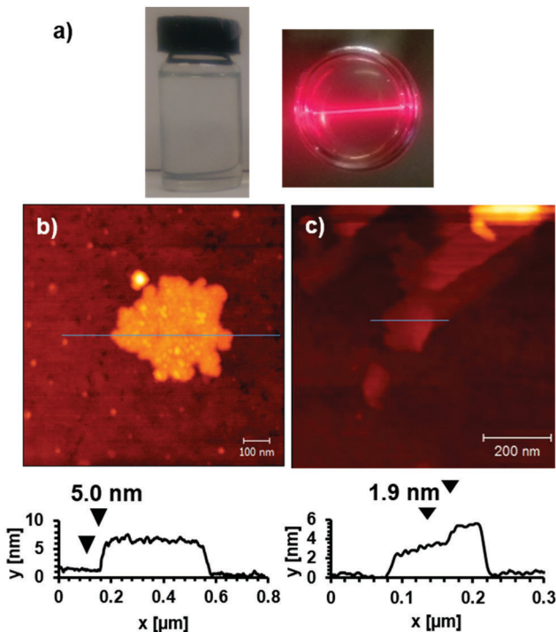
Fig. 2 (a) Images showing a suspension of \text{Cu}(\text{1}) nanosheets in DMF with characteristic Tyndal Scattering of laser light. AFM images and height profiles corresponding to blue lines for nanosheets formed by exfoliation of (b) \text{Zn}(\text{1}) in DMF (c) \text{Cu}(\text{1}) in \text{H}_2\text{O} .
