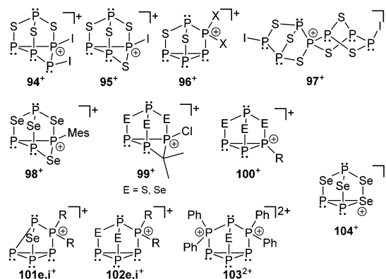
Fig. 17 Selected cationic polyphosphorus–chalcogen cages 94 ^+ – 103 ^{2+} ( E = S, Se ) comprising bonding motif J; cation 104 ^+ has been included since it represents the first binary SeP–cation and is related to the other cations.
