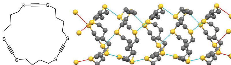
Scheme 6 Supramolecular nanotubes constructed from 1,4,9,12,17,20-hexathiacyclotetracos-2,10,18-tri- yn -4-one. 41
