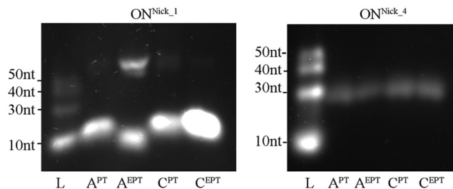
Fig. 5 Incorporation of modified dNTPs in NEAR using Nick_1A, Nick_1C and Nick_4A(4C) templates. L: DNA ladder; A PT : product of NEAR with dA PT TP, dCTP, dGTP, dTTP; A EPT : product of NEAR with dA EPT TP, dCTP, dGTP, dTTP; C PT : product of NEAR with dC PT TP, dATP, dGTP, dTTP; C EPT : product of NEAR with dC EPT TP, dATP, dGTP, dTTP.
