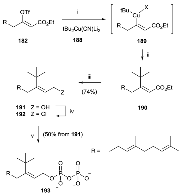
Scheme 33 Reagents and conditions: (i) \text{tBu}_2\text{Cu}(\text{CN})\text{Li}_2 , -78^\circ\text{C} . (ii) Reductive elimination. (iii) DIBALH, PhMe, -78^\circ\text{C} . (iv) NCS, \text{Me}_2\text{S} , \text{CH}_2\text{Cl}_2 . (v) (\text{Bu}_4\text{N})_3\text{HP}_2\text{O}_7 , \text{CH}_3\text{CN} .
