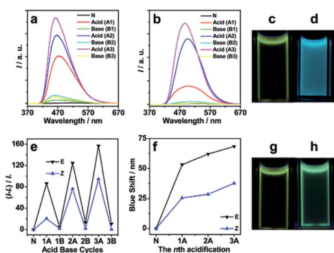
Fig. 3 Fluorescence spectra of the solutions of E -2DBA-TPE (a) and (b) Z -2DBA-TPE mixed with 4DB24C8-TPE, respectively, under three acid-base reaction cycles. (e) The plots of fluorescence intensities and (f) the blue shifts of E -2DBA-TPE and Z -2DBA-TPE in the THF solutions upon successive treatments with HCl and NaOH. As revealed by the photographs under UV irradiation at 365 nm, the solutions of E -2DBA-TPE (d) and Z -2DBA-TPE (h) mixed with 4DB24C8-TPE showed remarkable fluorescence enhancements and impressive blue shifts upon the third acid treatment compared to their respective original solutions (c and g). The concentrations of E/Z -2DBA-TPE and 4DB24C8-TPE were controlled at 1.0 and 0.5 mM, respectively. Here, N, A and B denote the neutral solution and its acid and base treatments, respectively. 1, 2 and 3 denote the sequence of the acid-base cycle.
