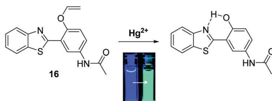
Scheme 17 Vinyl-ether protected ES IPT probe 16 , a species that proved useful for the selective detection of \text{Hg}^{2+} . Measurement conditions: PBS (pH 7.4) containing 1% ACN. Adapted with permission from ( Org. Lett. , 2011, 13 , 3422–3425). Copyright (2011) American Chemical Society.
