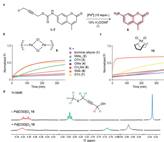
Fig. 1 Functional group screening to determine strategy used to bifunctionalize propargyl carbamates. (a) Decaging reaction of substituted propargyl carbamate protected 7-amino-4-methylcoumarin 1–7 through reaction with palladium complexes. (b) Increase in fluorescence of decaging reactions over time. Propargyl carbamate protected fluorophore has quenched fluorescence which is restored upon decaging. The reactions were performed at 100 \mu\text{M} final concentration of the fluorophores, with 5 equiv. of allylpalladium(II) chloride dimer 9 . (c) Fluorescence screening performed with 10 equiv. Pd(COD)Cl 2 10 . The data were normalized with respect to 100 \mu\text{M} of free fluorophore (7-amino-4-methyl coumarin 8 ) plus the final concentration of the palladium complex (0.5 mM for 9 and 1 mM for 10 ). (d) 1 H NMR data supporting hypothesis of binding of Pd(COD)Cl 2 with methyl propargyl thioether motif.
