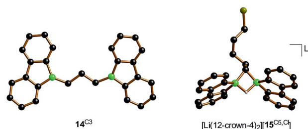
Fig. 4 Molecular structures of 14 C3 and of the terminally chlorine-substituted [\text{Li}(12\text{-crown-4})_2][15^{\text{C}5,\text{Cl}}] in the solid state. The solvent-separated [\text{Li}(12\text{-crown-4})_2]^+ cation, all t Bu groups, and all CH atoms are omitted for clarity.
