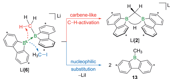
Scheme 9 The intermediate Li[6] can be interpreted as an adduct between the 9-borafluorenyl anion ( [\text{BFlu}]^- ) and 9-methyl-9-borafluorene ( 13 ). Intramolecular C-H insertion of the carbene-like [\text{BFlu}]^- furnishes Li[2] ; intermolecular nucleophilic attack on \text{H}_3\text{C-I} affords 2 equiv. of 13 . Carbon atoms marked with asterisks bear t Bu substituents.
