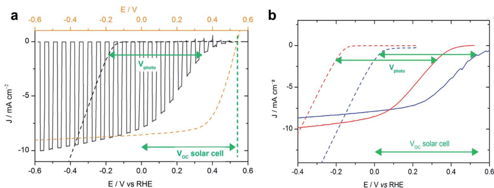
Fig. 4 (a) Voltammogram recorded at 50 \text{ mV s}^{-1} in 0.5 \text{ M H}_2\text{SO}_4 with chopped visible light for an ITO/PEDOT:PSS/P3HT:PCBM/LiF/Al/Ti- \text{MoS}_3 photocathode (black line, electrode area 0.32 \text{ cm}^2 ) and recorded at 5 \text{ mV s}^{-1} in 0.5 \text{ M H}_2\text{SO}_4 for an ITO- \text{MoS}_3 cathode (black dashed line, electrode area 0.28 \text{ cm}^2 ). Potentials are referred to the RHE (bottom axis). The current-voltage curve of an ITO/PEDOT:PSS/P3HT:PCBM/LiF/Al solar cell (orange dashed line, top axis) is shown for comparison. (b) Voltammogram recorded at 5 \text{ mV s}^{-1} in 0.5 \text{ M H}_2\text{SO}_4 for an ITO- \text{MoS}_3 cathode (red dotted line) and an ITO-Pt/C cathode (blue dotted line) and at 50 \text{ mV s}^{-1} with visible-light illumination ( 100 \text{ mW cm}^{-2} ) for an ITO/PEDOT:PSS/P3HT:PCBM/LiF/Al/Ti- \text{MoS}_3 photocathode (red line) and an ITO/PEDOT:PSS/P3HT:PCBM/LiF/Al/Ti-Pt/C photocathode (blue line). Reprinted with permission from Bourgeteau, et al. , ACS Appl. Mater. Interfaces , 7, 30, 16395–16403. Copyright (2015) American Chemical Society. 31
