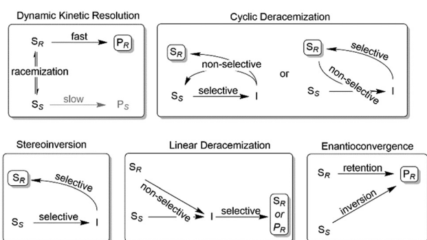
Scheme 2 Common deracemisation methods. S: chiral starting material such as an amine or alcohol, P: product, I: prochiral intermediate such as a ketone or an imine.
