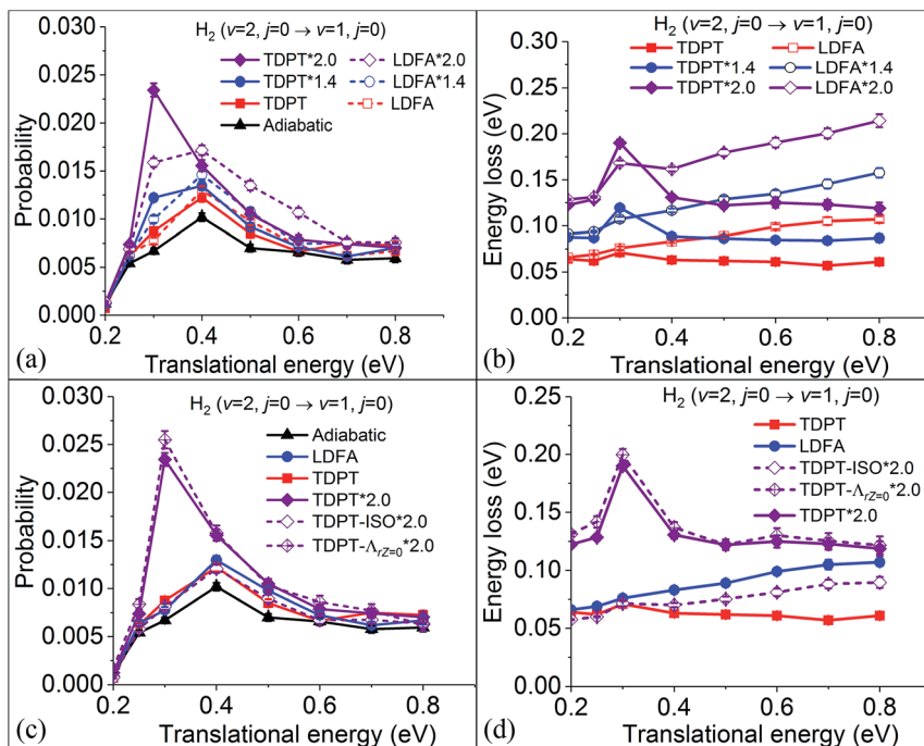
Fig. 4 (a) Vibrational deexcitation probabilities from H 2 (v = 2, j = 0) to H 2 (v = 1, j = 0) as a function of translational energy, with adiabatic dynamics (triangles), with electronic friction by LDFA (open symbols) and TDPT (solid symbols) models, and with 1.4 (circles) and 2.0 (diamonds) times larger friction coefficients. (b) Mean nonadiabatic energy losses for various simulations in panel (a). (c) On the basis of (a) but adding new data computed by removing anisotropy (TDPT-ISO*2) and the Z-r coupling term (TDPT- \Lambda_{rZ=0} *2.0) in the TDPT friction tensor. (d) Mean nonadiabatic energy losses for various simulations in panel (b).
