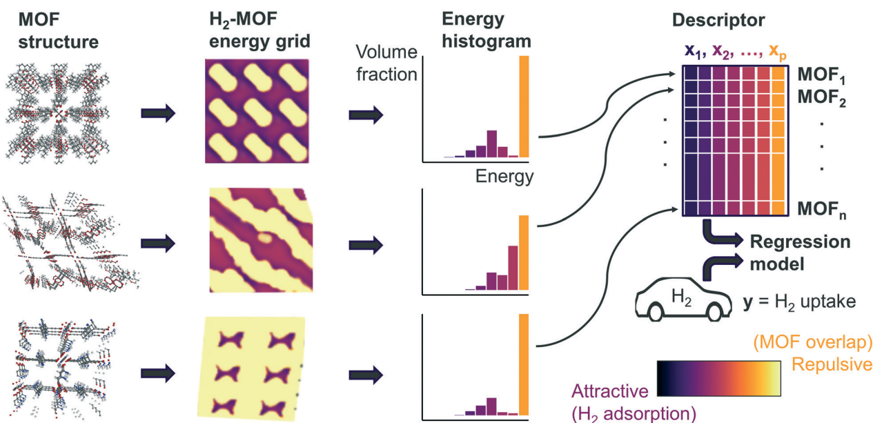
Fig. 1 Overall machine learning workflow. For each MOF, we sampled the potential energy distribution by calculating the energy of a hydrogen probe at grid points within the MOF unit cell, then summarized the distribution of energies as a histogram. Each bin in the resulting energy histogram is a feature in the regression model, which enables the model to capture effects from different attractive and repulsive regions of the MOF in predicting hydrogen deliverable capacity.
