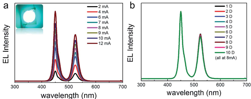
Fig. 9 (a) EL spectra of the CsPbBr 3 @Cs 4 PbBr 6 NC powder-based backlit LED under different currents; inset is the photograph of the backlit LED. (b) EL spectra of the CsPbBr 3 @Cs 4 PbBr 6 -based backlit LED lighted for 10 days under ambient conditions.
