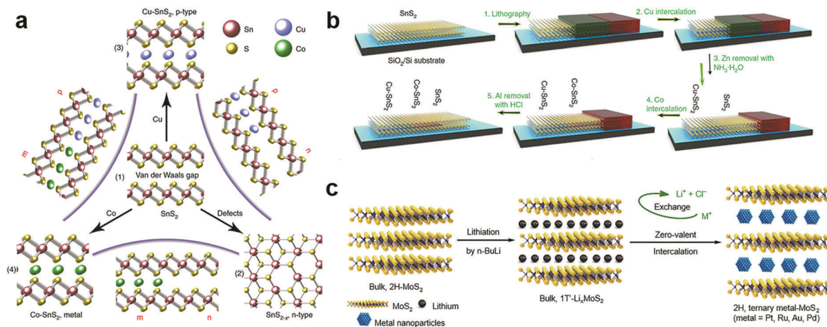
Fig. 11 Zerovalent interaction of MXs: (a) the zerovalent intercalation of SnS 2 by Cu and Co, enabling facile p, n, and metallic modulation. (b) The illustration of mask protected intercalation for fabricating lateral junctions, reprinted with permission from ref. 187, Copyright 2018 Nature Publishing group. (c) The lithium intercalation assisted zerovalent intercalation of noble metals into MoS 2 , reprinted with permission from ref. 36, Copyright 2017 Nature Publishing group.
