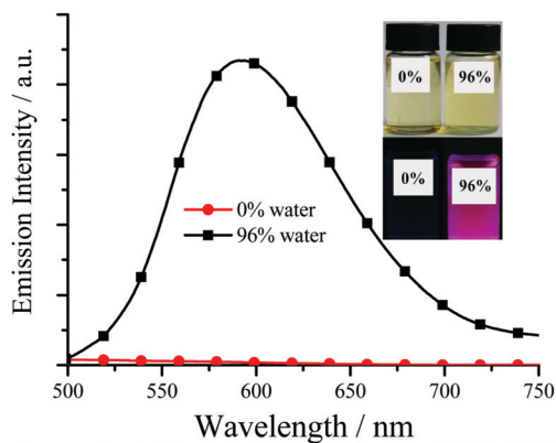
Fig. 3 Top: Emission spectra of ppy-Pt-3-Cl-(S,S)Cy in THF and THF/water ( 2.0 \times 10^{-5} mol \text{dm}^{-3} ). Inset: Their photographs under room light and 360 nm UV light. Bottom: Transmission electron microscopy of ppy-Pt-3-Cl-(S,S)Cy (THF/water, 96% water) on carbon-coated copper grids after solvent evaporation.
