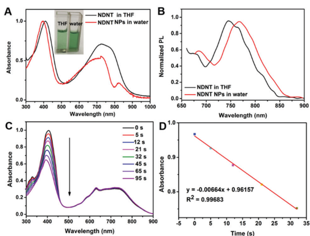
Fig. 1 (A) Normalized absorbance of NDNT in THF and NPs in water; (B) normalized PL of NDNT in THF and NPs in water; (C) degradation of DPBF under the presence of NDNT in DCM with laser irradiation; (D) linear fitting of the degradation of DPBF.
