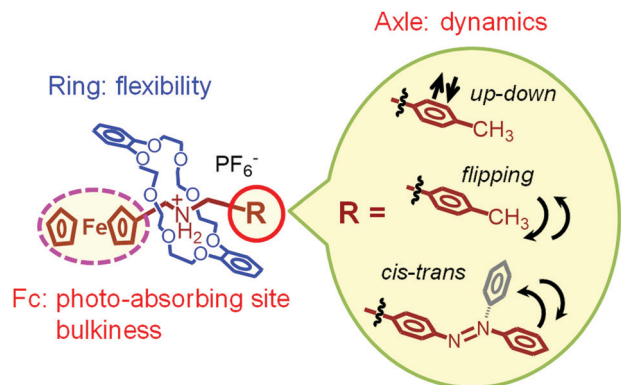
Fig. 20 Schematic illustration of the molecular motions and functions of ferrocene-containing pseudorotaxanes.
