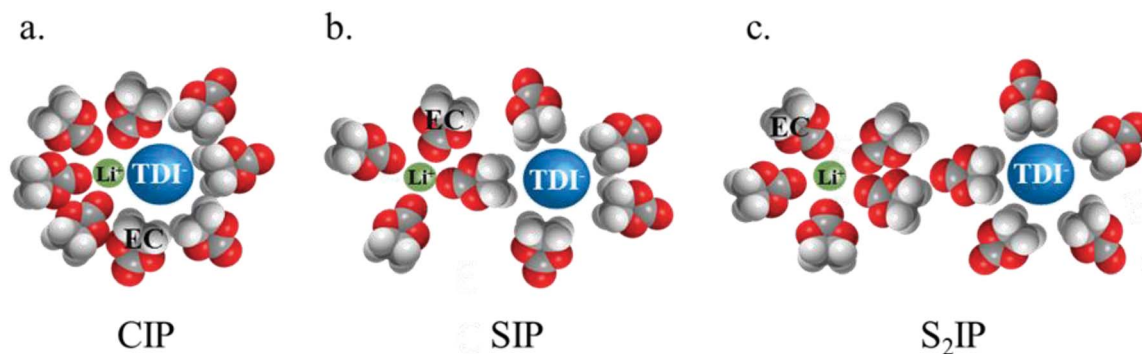
Fig. 1 Schematic view of different types of ion-pairs, (a) contact ion-pair (CIP), (b) solvent-shared ion-pair (SIP) and (c) solvent separated ion-pair ( \text{S}_2\text{IP} ) in the case of the \text{LiTDI} salt dissolved in EC.
