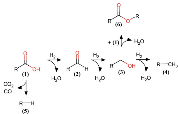
Fig. 6 Reaction network for the Mo-based catalysts in the HDO of palmitic acid ( \text{R} = \text{C}_{15}\text{H}_{31} ). (1) Palmitic acid, (2) hexadecanal, (3) 1-hexadecanol, (4) n -hexadecane, (5) n -pentadecane and (6) cetyl palmitate.
