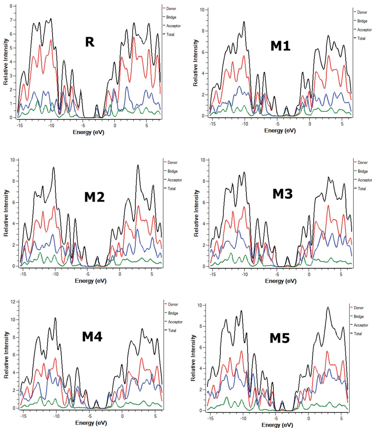
Fig. 5 The DOS around the HOMOs and LUMOs of reference R and the designed molecules M1 – M5 at B3LYP/6-311G(d,p) level of theory.
