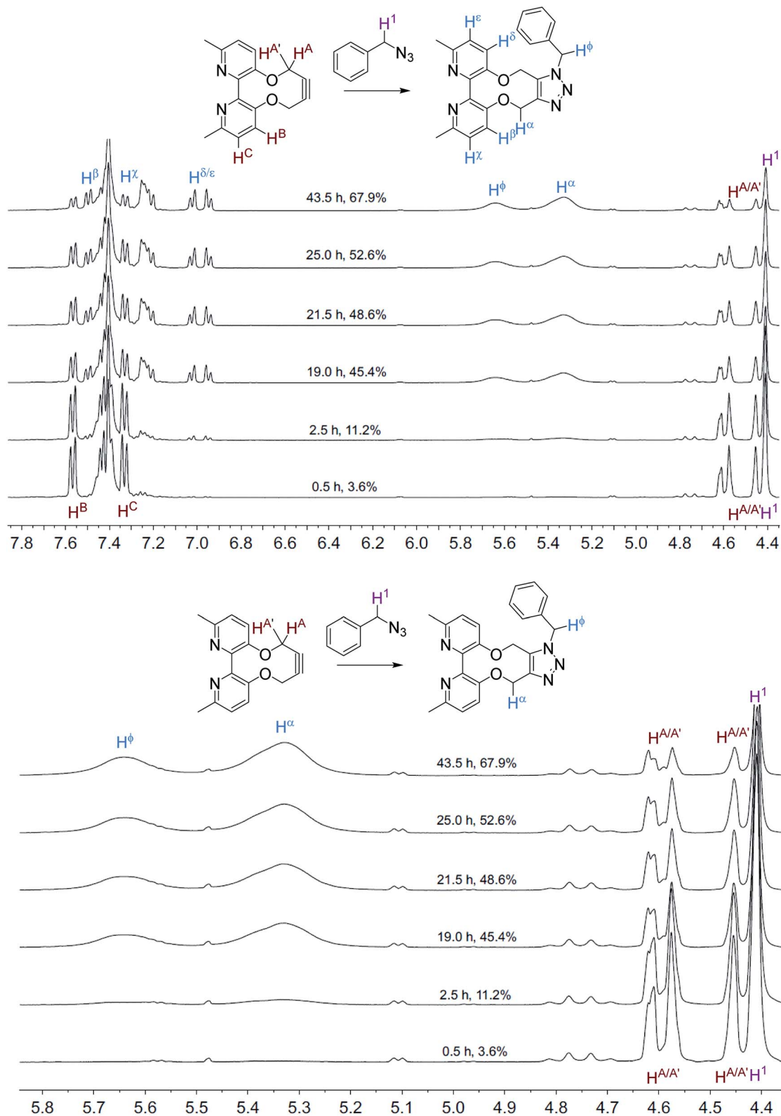
Fig. 2 Overlaid 1 H NMR spectra (400 MHz, CD 3 CN, 298 K) for the cycloaddition reaction in Scheme 3 without added ZnCl 2 .
