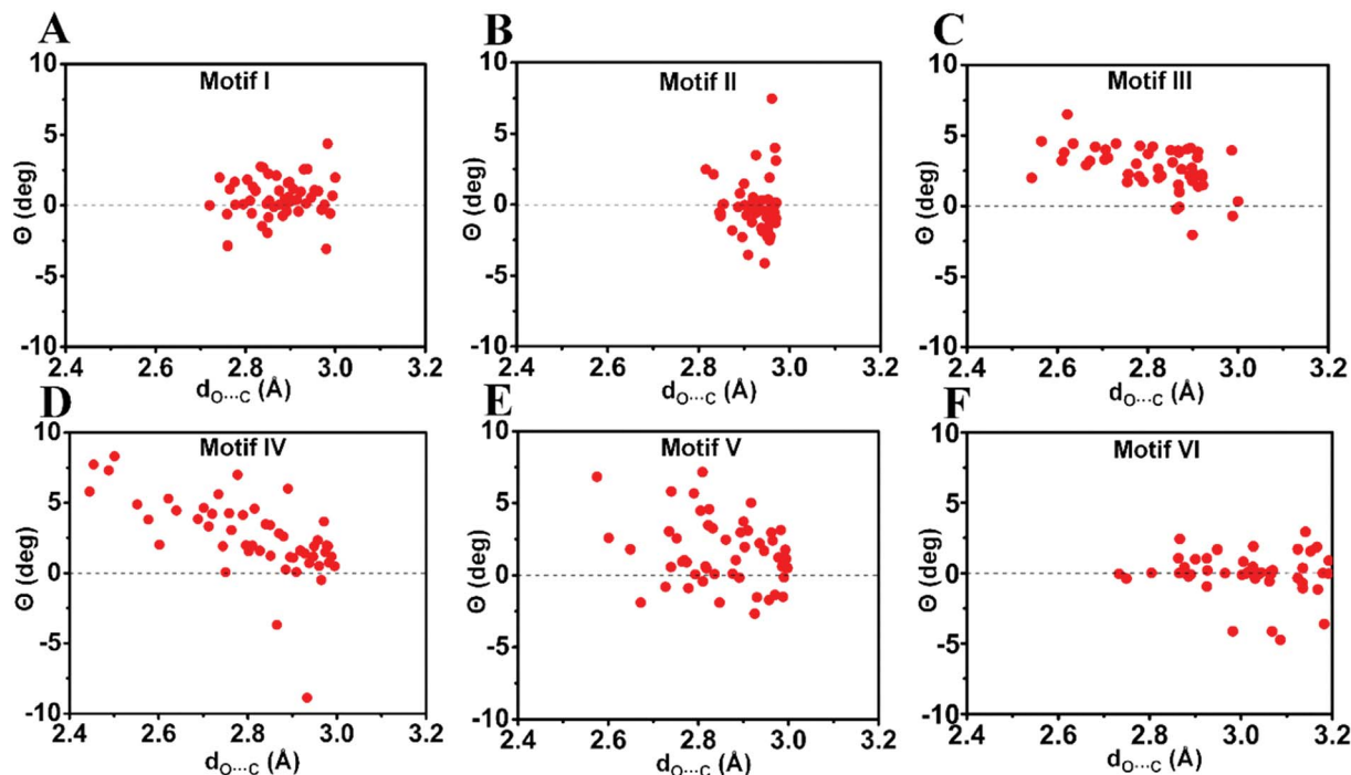
Fig. 7 Pyramidity ( \theta ) of the acceptor carbonyl carbon in motifs I–VI. (A)–(F) Motifs (I)–(VI). Only molecules with d_{O\dots C} \leq 3.0 \text{ \AA} [ d_{O\dots C} \leq 3.2 \text{ \AA} for motif VI] were considered. See ESI† for details.
