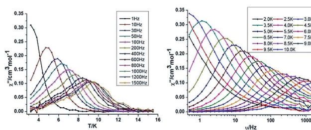
Fig. 6 Temperature (left) and frequency (right) dependence under 1000 Oe dc field of the out-of-phase ( \chi'' ) for compound 8 \{Al_2Dy_{0.18}Y_{1.82}\} .
