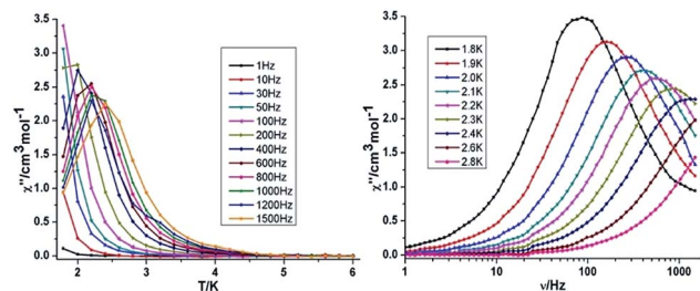
Fig. 4 Temperature (left) and frequency (right) dependence under zero dc field of the out-of-phase ( \chi'' ) for compound 3 \{Mn_2Dy_2\} .
