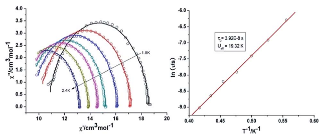
Fig. 5 Cole–Cole plots at indicated temperature (left) and \tau vs. T^{-1} plot in zero dc field (right) for 3 \{Mn_2Dy_2\} .
