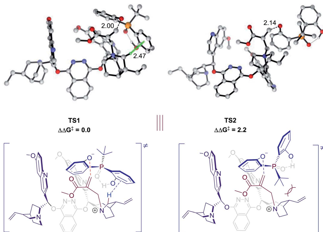
Fig. 2 Transition state structures and relative free energies (in kcal mol -1 ) for desymmetrization catalyzed by 4f. Noncritical hydrogen atoms have been omitted for clarity. The C-H \cdots\pi interaction in TS1 is highlighted.
