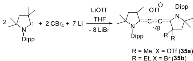
Fig. 8 Synthesis of di-cAAC stabilized \text{C}_2^+ .
