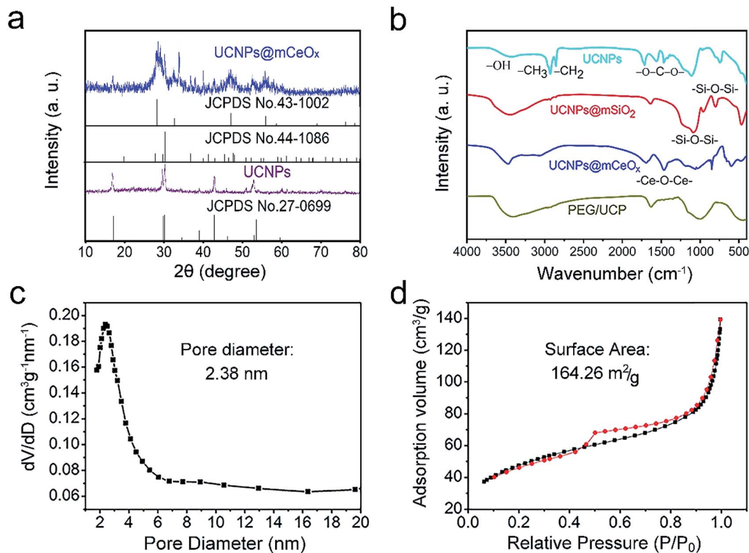
Fig. 2 XRD patterns of UCNP@mCeO x (the standard lines of \beta -NaGdF 4 , CeO 2 and Ce 2 O 3 are supplied for comparison) (a) and FT-IR spectra of OA-UCNPs, UCNP@mSiO 2 , UCNP@mCeO x and PEG/UCP (b). The pore-size distribution (c) and N 2 adsorption/desorption isotherm (d) of UCNP@mCeO x .
