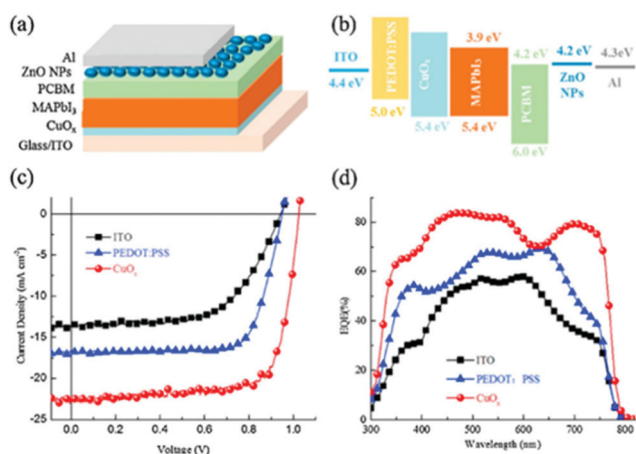
Fig. 22 (a) Schematic of the CuO_x/ZnO based device structure; (b) energy-level diagram of the corresponding device; (c) J - V curves and (d) EQE spectra of the PVSCs without or with different HTLs. 135
