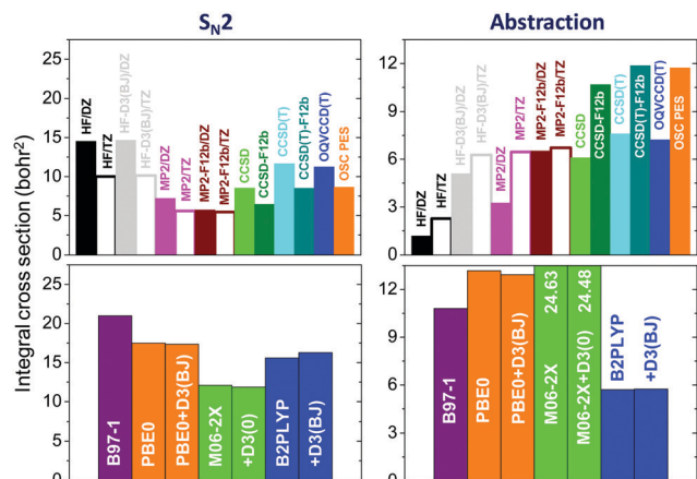
Fig. 11 Cross sections for the F^- + CH_3I S_N2 and proton-abstraction reactions obtained by quasiclassical trajectory computations on various ab initio - and DFT-based analytical PESs at a collision energy of 35.3 \text{ kcal mol}^{-1} . 71 DZ and TZ denote aug-cc-pVDZ and aug-cc-pVTZ basis sets, respectively, the CCSD, CCSD-F12b, CCSD(T), CCSD(T)-F12b, and OQVCCD(T) methods are used with DZ and the DFT methods are used with TZ basis sets. D3(BJ) and D3(0) denote additive dispersion corrections 135,136 and the all-electron CCSD(T)-F12b/TZ-quality OSC PES is taken from ref. 45.
