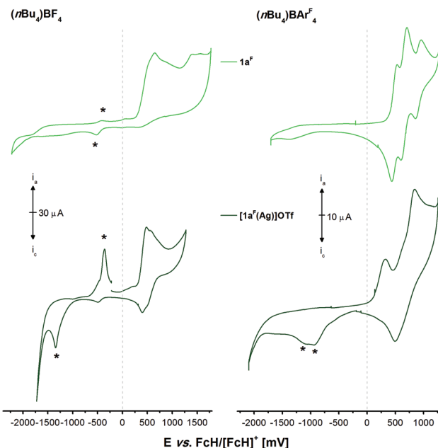
Fig. 9 Cyclic voltammograms of 1 mmol L -1 1a F (light green) and [1a F (Ag)]OTf (dark green) in 0.1 mol L -1 supporting electrolyte solutions (( n Bu 4 N)BF 4 (left) and ( n Bu 4 N)BARF 4 (right) in CH 2 Cl 2 ). Traces have been recorded at 100 mV s -1 (working electrode: glassy carbon, counter electrode: Pt wire) at room temperature. The second of three cycles are shown and asterisks (*) mark oxidation/reduction events which depend on prior oxidation in the first cycle ( cf. Fig. S66 and S67†).
