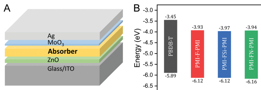
Fig. 6 (A) Device architecture of the fabricated solar cells and (B) energy diagram of PMI-F-PMI ( 3a ), PMI-FSi-PMI ( 3b ), PMI-FN-PMI ( 3c ) and PBDB-T . The HOMO/LUMO levels were determined by cyclic voltammetry.
