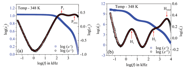
Fig. 1 Frequency dependence of the real ( \varepsilon' ) and imaginary ( \varepsilon'' ) parts of the permittivity for compound 1/7 : in (a) HG or planar and (b) HT or homeotropic sample configurations. Red solid curves represent the fit to the data points with eqn (3).
