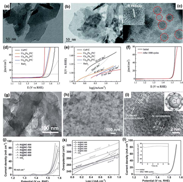
Fig. 22 TEM images of (a) Co 0.7 Fe 0.3 -MOF nanosheets and (b) Co 0.7 Fe 0.3 P/C nanosheets. (c) HRTEM image of Co 0.7 Fe 0.3 P/C nanosheets. (d) LSV curves and (e) the corresponding Tafel plots of Co 1-x Fe x P/C nanosheets and commercial RuO 2 catalyst in 1 M KOH solution. (f) Polarization curves of the Co 0.7 Fe 0.3 P/C catalyst before and after 1000 potential cycles. Reproduced with permission. 197 Copyright ©2018 The Royal Society of Chemistry. (g) TEM image of Ni-BDC nanosheets. (h) SEM and (i) HRTEM images of Ni@NC. (j) The OER polarization curves and (k) the corresponding Tafel plots of various Ni@NC samples and commercial IrO 2 catalyst in 1.0 M KOH solution. (l) Polarization curves of the Ni@NC-800 catalyst before and after 1000 potential cycles. The inset of (l) is the chronoamperometric curve at 1.52 V (vs. RHE). 198 Copyright©2017 WILEY-VCH Verlag GmbH & Co. KGaA.
