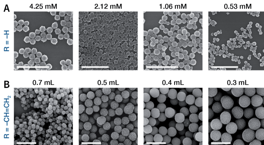
Fig. 36 SEM images of imine-linked COFs prepared in \text{CH}_3\text{CN} at room temperature. (A) TAPB-PDA COF with particle sizes of 200, 260, 290, and 330 nm prepared at varying aryltriamine monomer concentrations. Scale bar: 2 \mu\text{m} . Adapted with permission. 219 Copyright 2019, The Royal Society of Chemistry. (B) TAPB-DVA COF with particle sizes of 450, 800, 1000, and 1300 nm synthesized at different volumes of acetic acid. Scale bar: 2 \mu\text{m} . Adapted with permission. 222 Copyright 2019, American Chemical Society.
