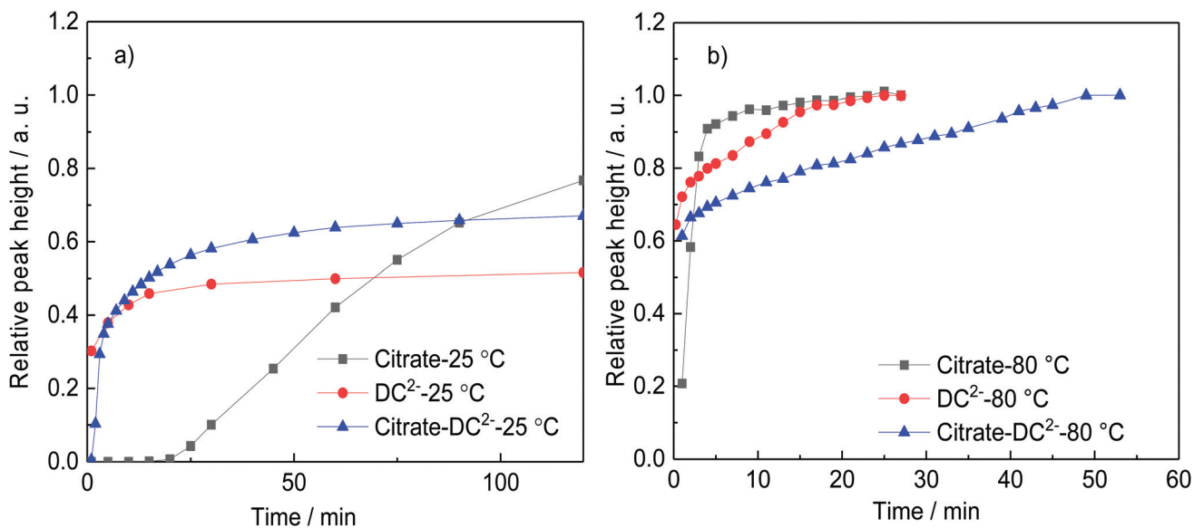
Fig. 1 Comparison of the rate of formation of gold nanoparticles (represented by the relative height of the absorption peak) using sodium citrate or DC 2- as a reducing agent at a. 25 °C and b. 80 °C. Conditions: [HAuCl 4 ]: 0.25 mM, pH: 4.8–4.9, reducing agent: [sodium citrate]: 2.5 mM, [DC 2- ]: 2.5 mM; or [sodium citrate] 2.5 mM + [DC 2- ] 2.5 mM, as in experiments A–F (Table 1).
