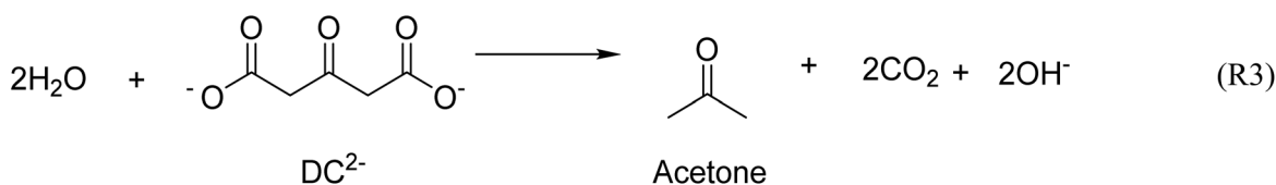
Scheme 2 Decomposition of DC 2- . 13
