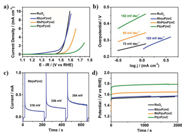
Fig. 2 Electrocatalytic performance for the OER in 0.1 M KOH solution. (a) LSV polarization curves of commercial \text{RuO}_2 , Rh(nP)/nC, RhPt(nP)/nC and Pt(nP)/nC at a scan rate of 5\text{ mV s}^{-1} . (b) Corresponding Tafel plots. (c) Representative 200 seconds potential steps of Rh(nP)/nC at overpotentials of 0.318 V, 0.336 V and 0.354 V, respectively. (d) Chronopotentiometry curves recorded at a current density of 2\text{ mA cm}^{-2} . The potentials were corrected for iR drop and calibrated to RHE.
