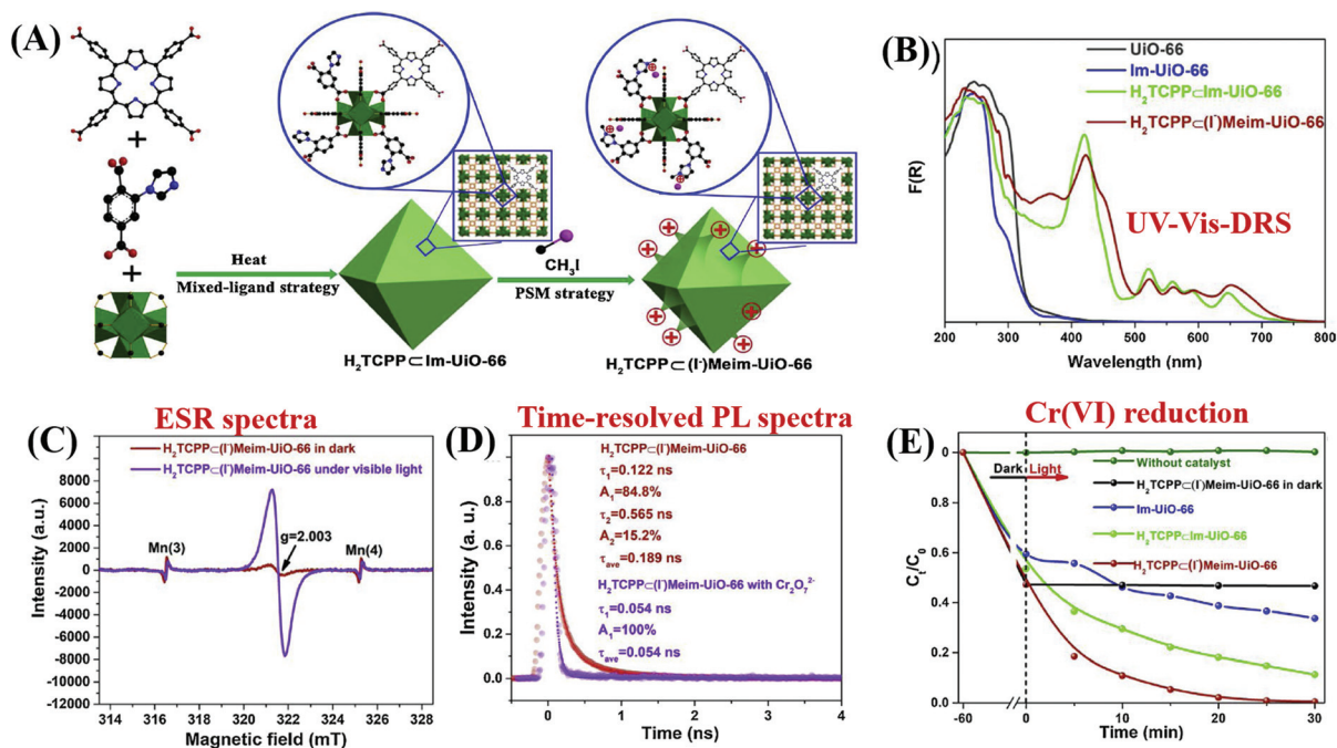
Fig. 36 (A) Schematic processes for the preparation of H_2TCPP-(I)Meim-UiO-66 ; (B) UV-vis-DRS of different samples; (C) ESR analyses of H_2TCPP-(I)Meim-UiO-66 with Mn as an internal standard; (D) time-resolved PL spectra of H_2TCPP-(I)Meim-UiO-66 suspensions with and without the presence of Cr_2O_7^{2-} at an emission wavelength of 650 nm ( \lambda_{ex} = 400 nm); (E) photocatalytic reduction of Cr(VI) by different samples under visible light irradiation. Adapted with permission from ref. 279, © 2019 Elsevier B.V.
