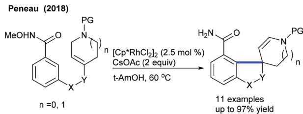
Scheme 97 Synthesis of spiro[pyridine] derivatives.
