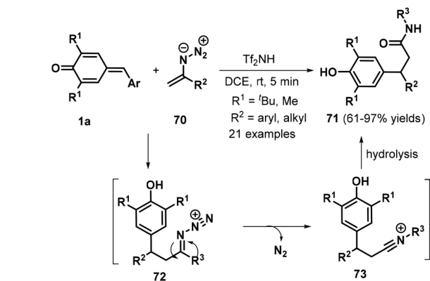
Scheme 16 \text{Tf}_2\text{NH} -Catalyzed rearrangement of p -QMs.
