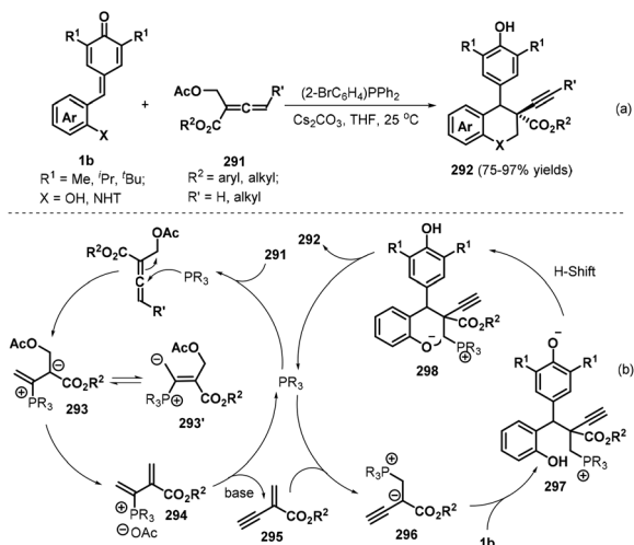
Scheme 64 [4 + 2] annulation of p -QMs with allenates.
