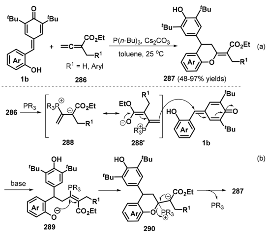
Scheme 63 Phosphine-catalyzed [4 + 2] annulation of p -QMs.
