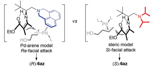
Scheme 43 Asymmetric allylation using Pd-primary amine co-catalysis.
