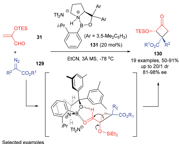
Scheme 37 Tandem cyclopropanation/semipinacol rearrangement.
