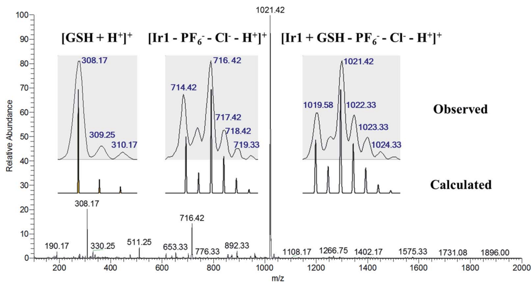
Fig. 1 ESI-MS spectrum with the isotopic distribution of the solution sample from the reaction of Ir1 (1 mM) and GSH (10 mM) in CH_3OH/H_2O (v/v, 1 : 1) after incubation for 6 h at 310 K. The assignments for the peaks are listed in the inset.
