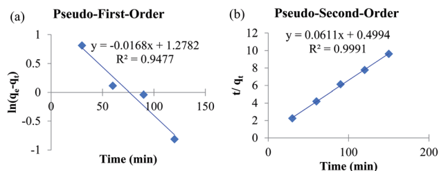
Fig. 6 Adsorption kinetics of MOF-801 as (a) pseudo-first-order and (b) pseudo-second-order for fluoride adsorption. Test conditions: adsorbent ( 1 \text{ g L}^{-1} ) and fluoride solution (20 mL).
