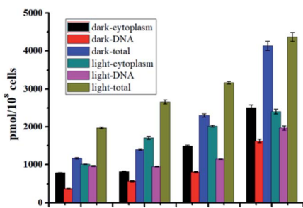
Fig. 5 Uptake levels of 1–4 (5 \mu\text{M} ) by S. aureus measured by ICP-MS.
